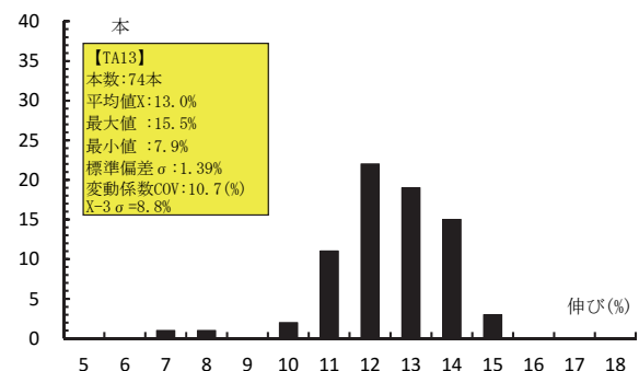
(a) 溶接試験片
